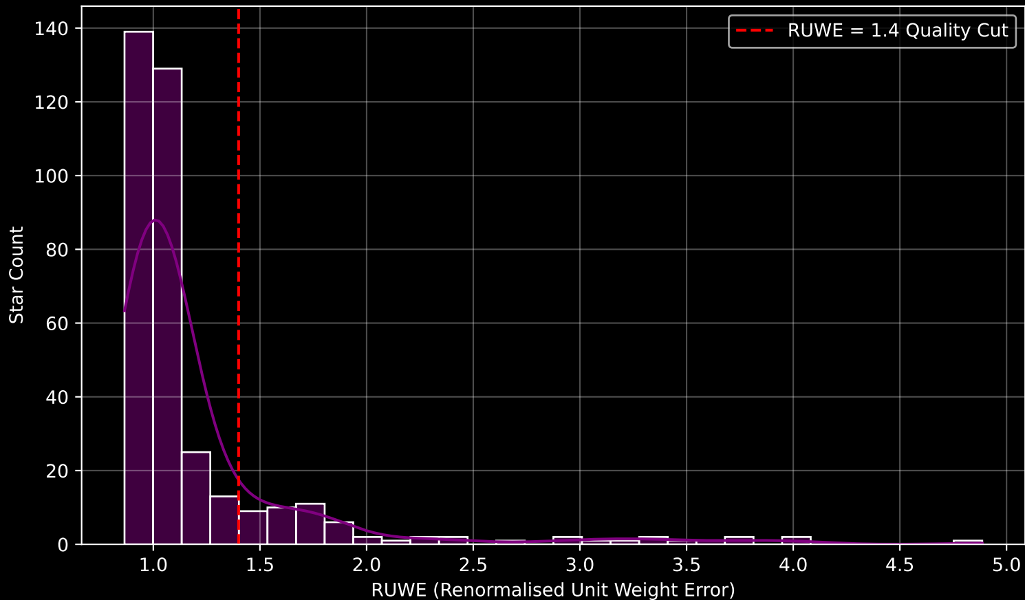
GALAH DR4 Field [6681] RUWE Distribution (n= 363)
