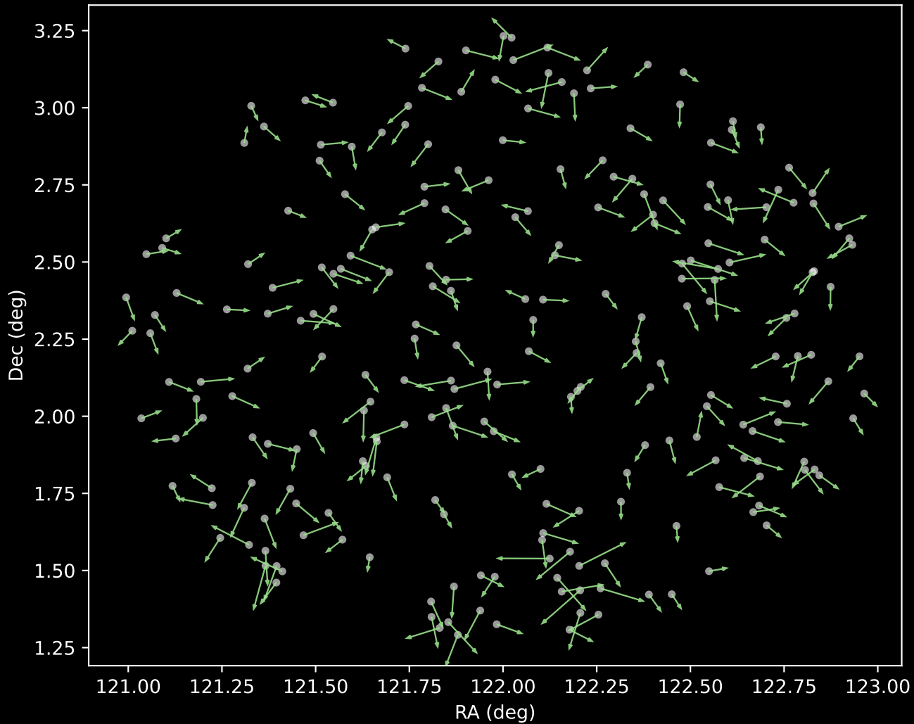
GALAH DR4 Cluster 5 Proper Motion Vectors (n=241)
