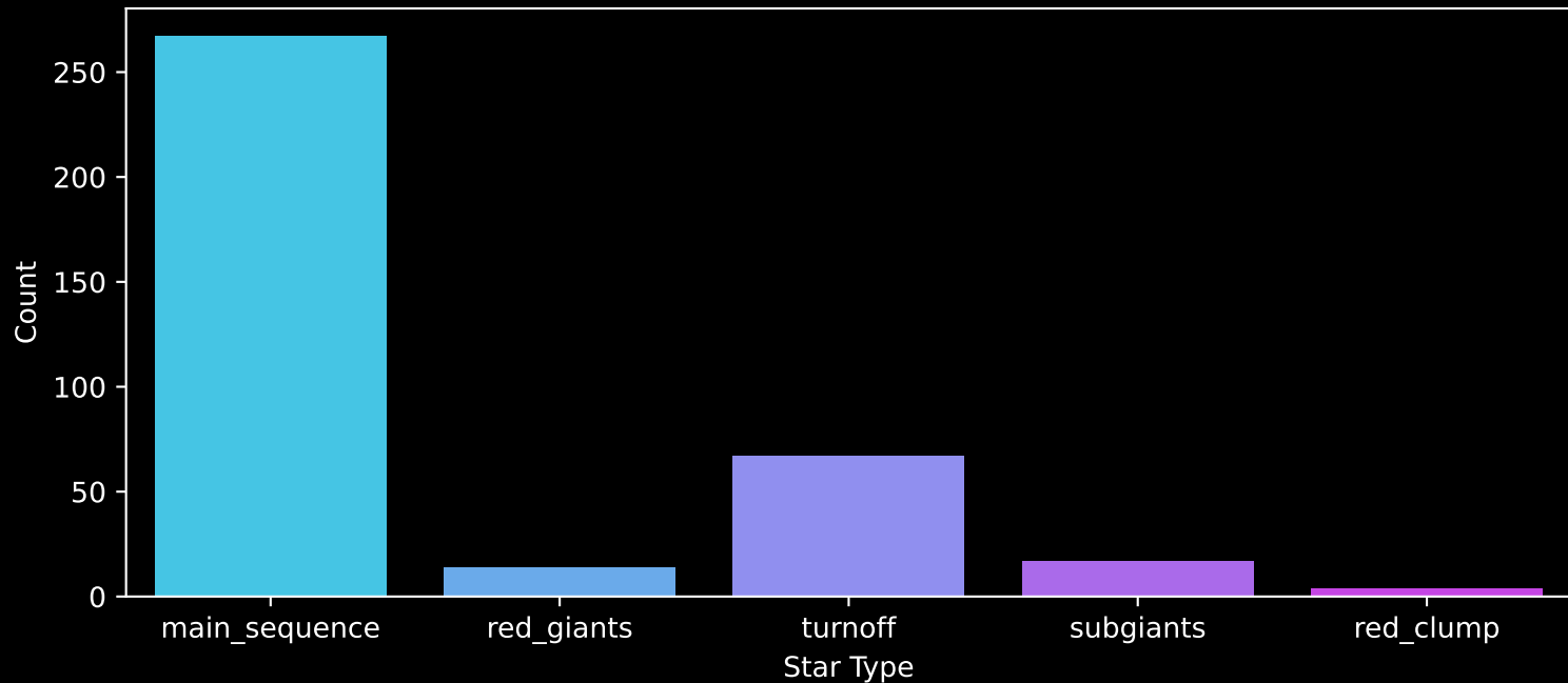
GALAH DR4 Field: [6681] Count plot of Star Type
