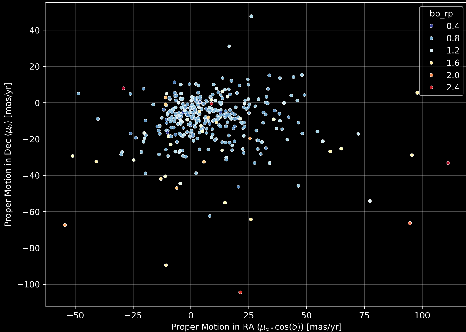
GALAH DR4 Field: [6681] Proper Motion Diagram (n= 369)
